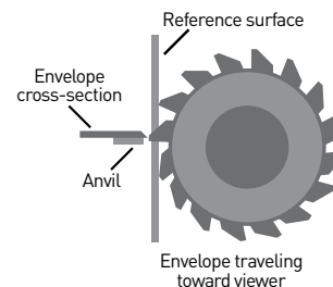
The unique milling cutter produces a soft, feathered edge.
